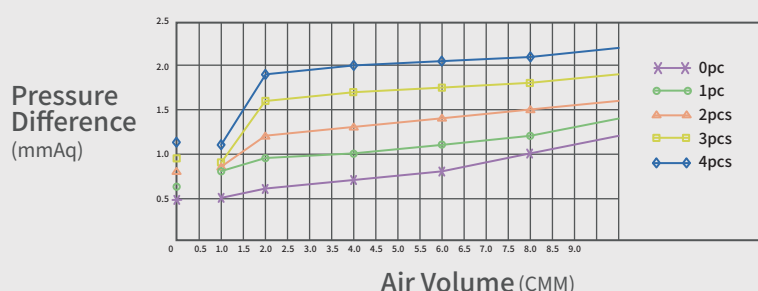
Performance Curve of Counterweights
